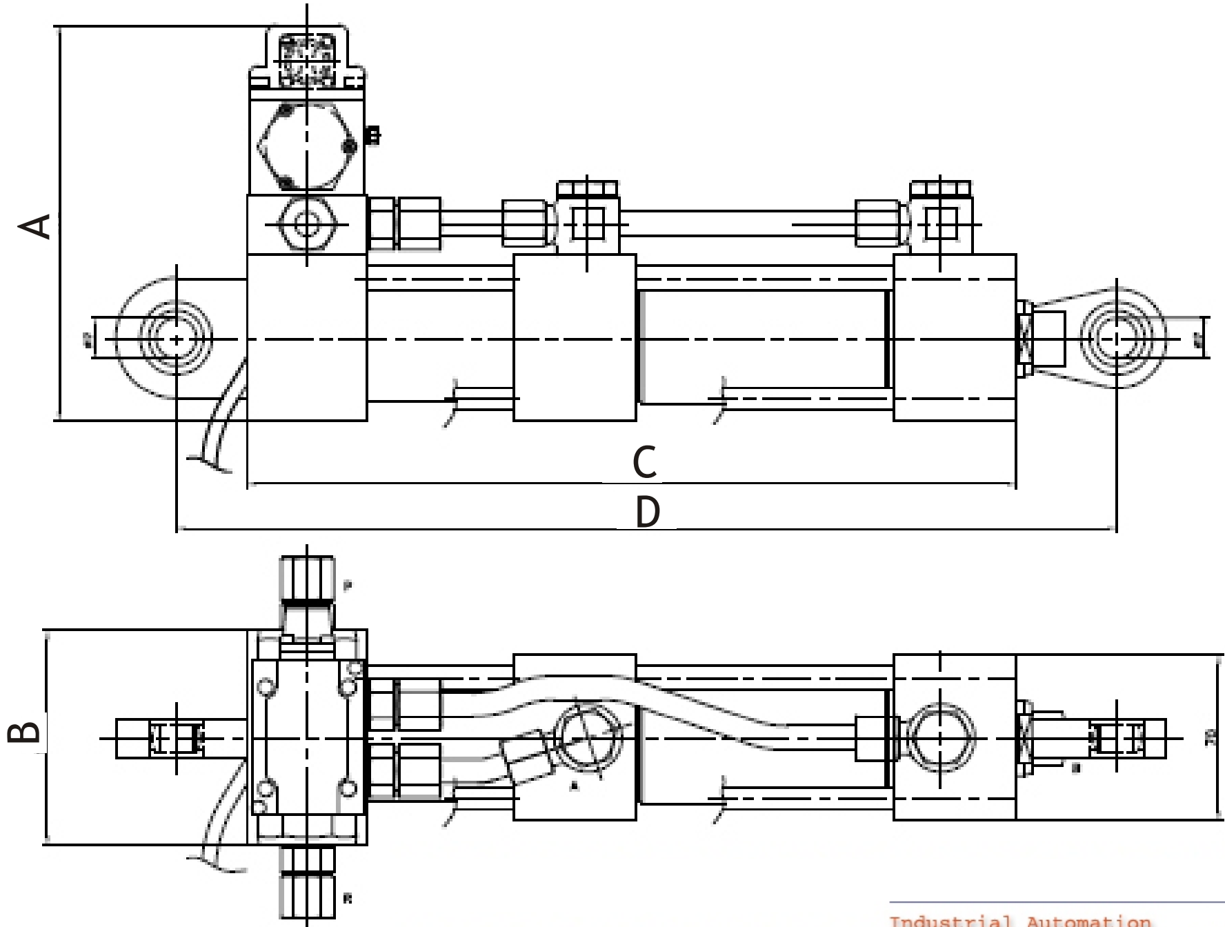
Hydraulic cylinder with servo valve and built in position transducer
